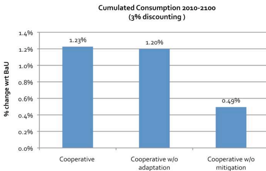
Figure 11: Global welfare
