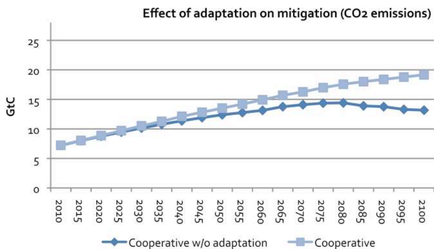
Figure 10: CO2 emissions
