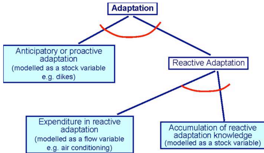
Figure Al.1: The adaptation tree in the AD_WITCH model
